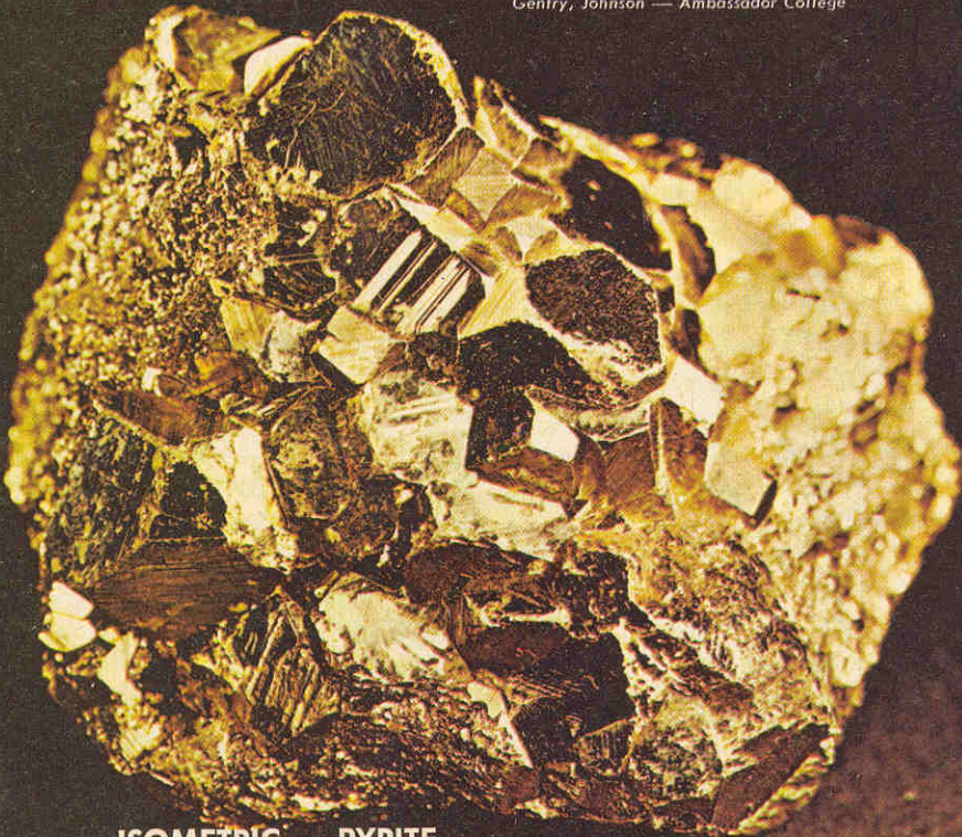
ISOMETRIC — PYRITE
